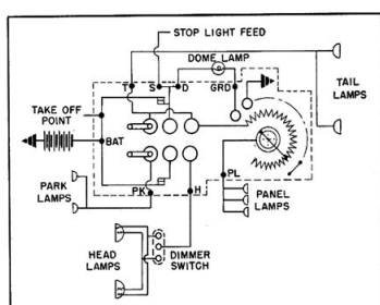
Fig. 3—Lighting Switch Circuit Diagram
